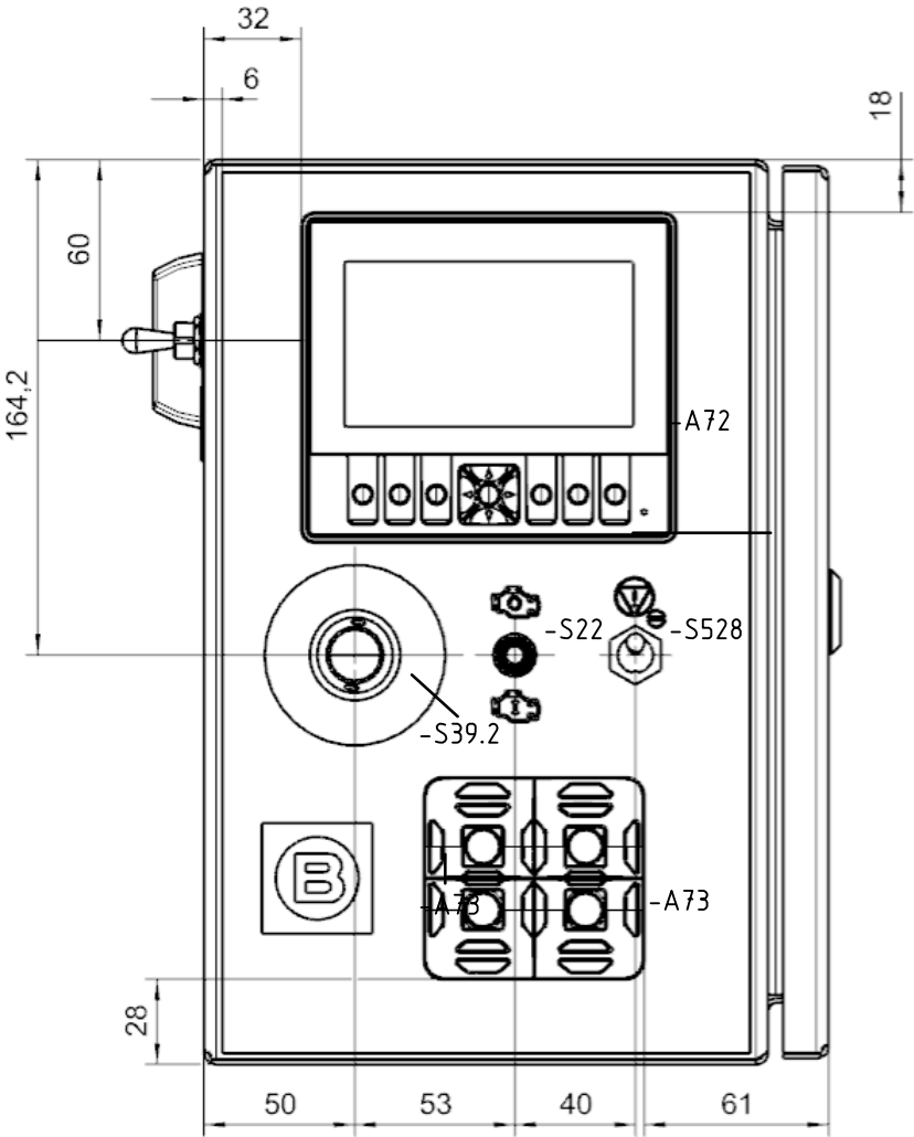
ANSICHT VON LINKS VIEW FROM LEFT SIDE
